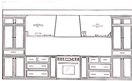
ELEVATION 1 - KITCHEN SCALE: 1/2" = 1'-0"
