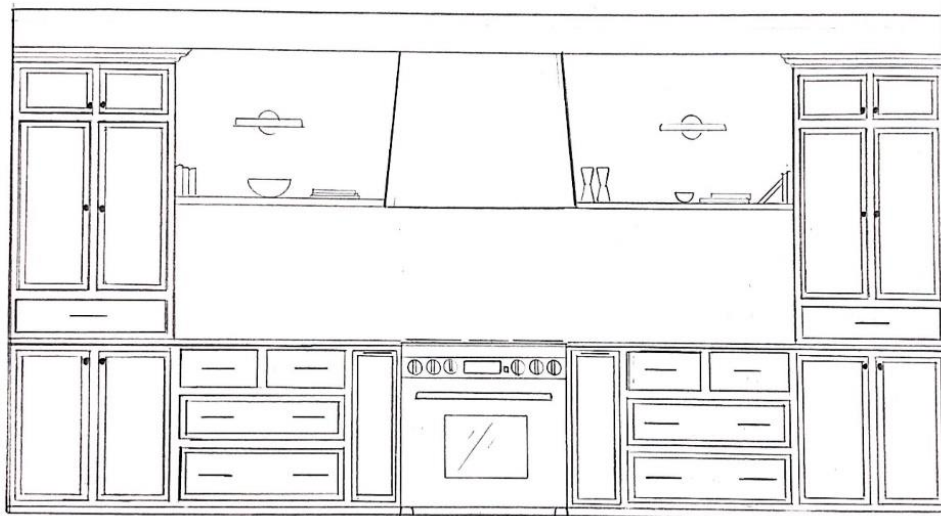
ELEVATION 1 - KITCHEN SCALE: 1/2" = 1'-0"
